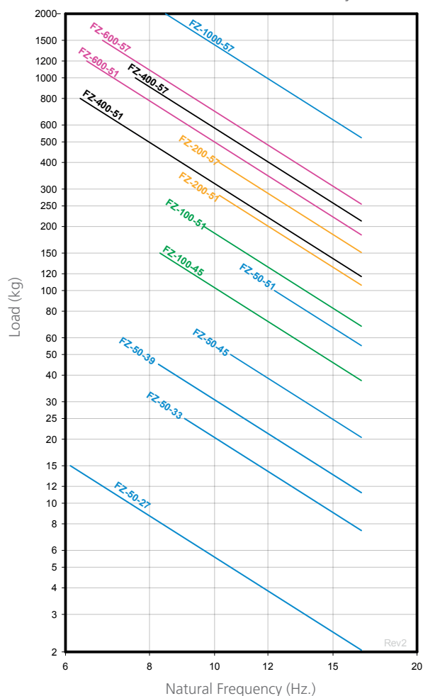
NATURAL FREQUENCY AMC MECANOCAUCHO® FZ + Sylomer®
