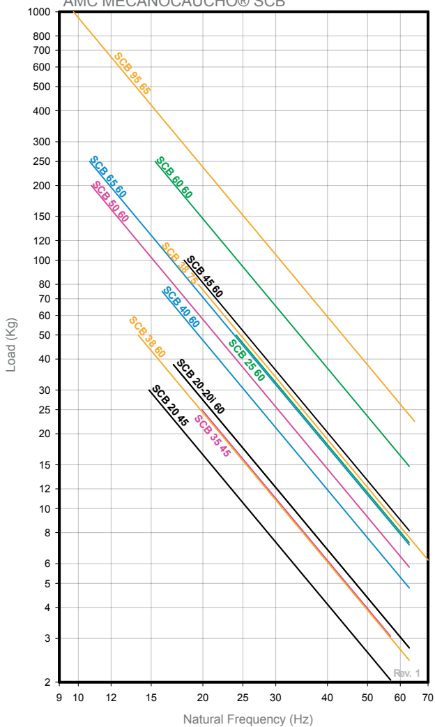
NATURAL FREQUENCY AMC MECANOCAUCHO® SCB
