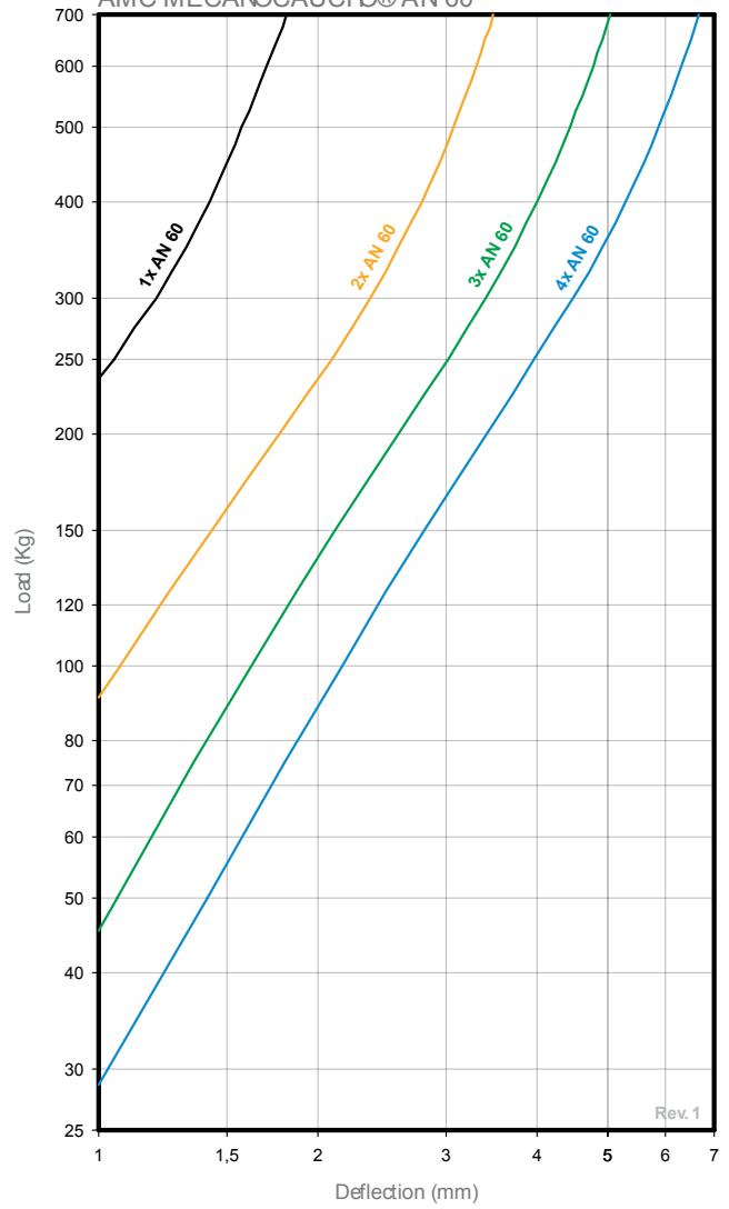
LOAD DEFLECTION GRAPH AMC MECANOCAUCHD® AN 60
