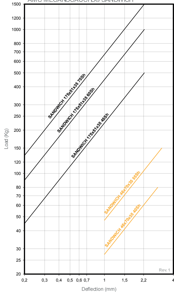
LOAD DEFLECTION GRAPH AMC MECANOCAUCHO® SANDWICH
