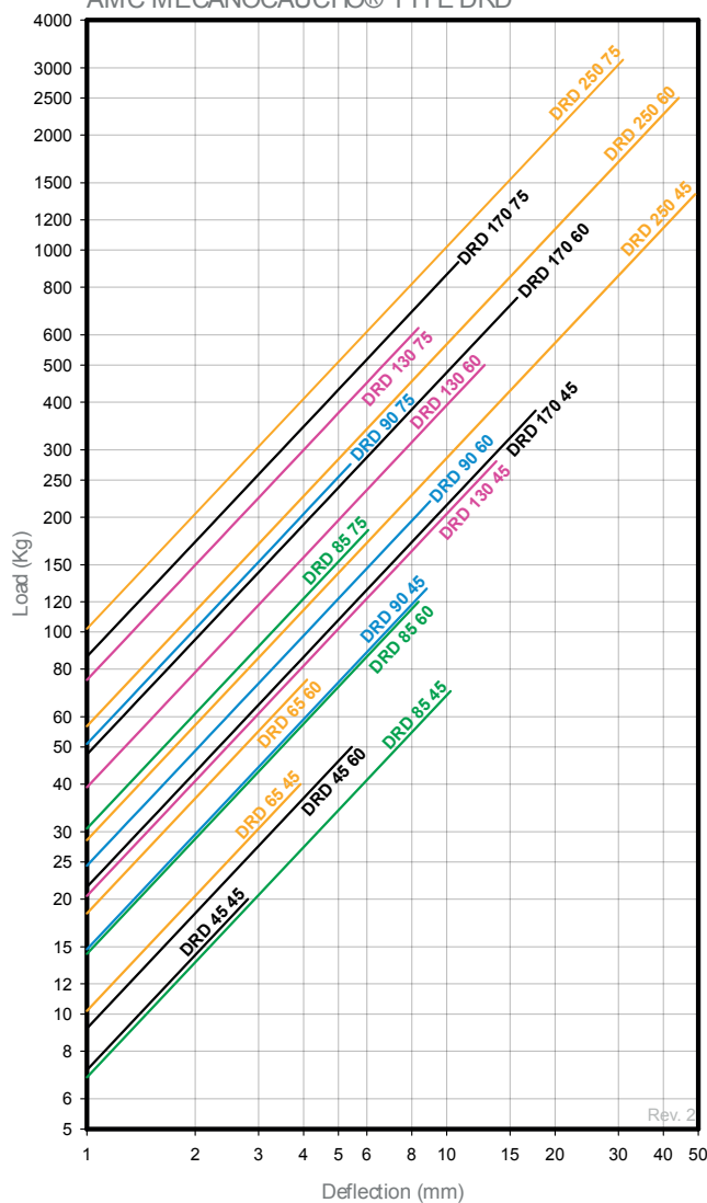
LOAD DEFLECTION GRAPH AMC MECANOCAUCHO® TYPE DRD
