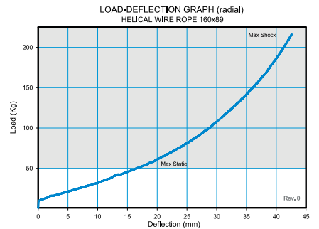
TYPE 160x89
