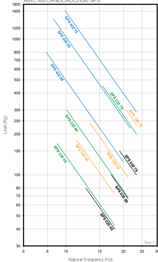
NATURAL FREQUENCY AMC MECANOCAUCHO® SPS
