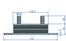
Sandwich-175x51x35
