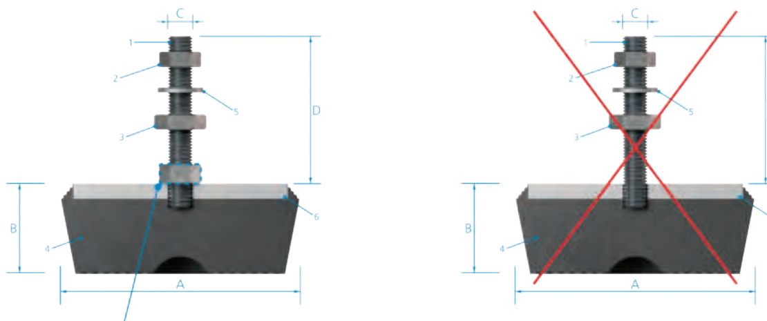
This nut spreads the load on the bell and avoids tensioning the below welded insert.
