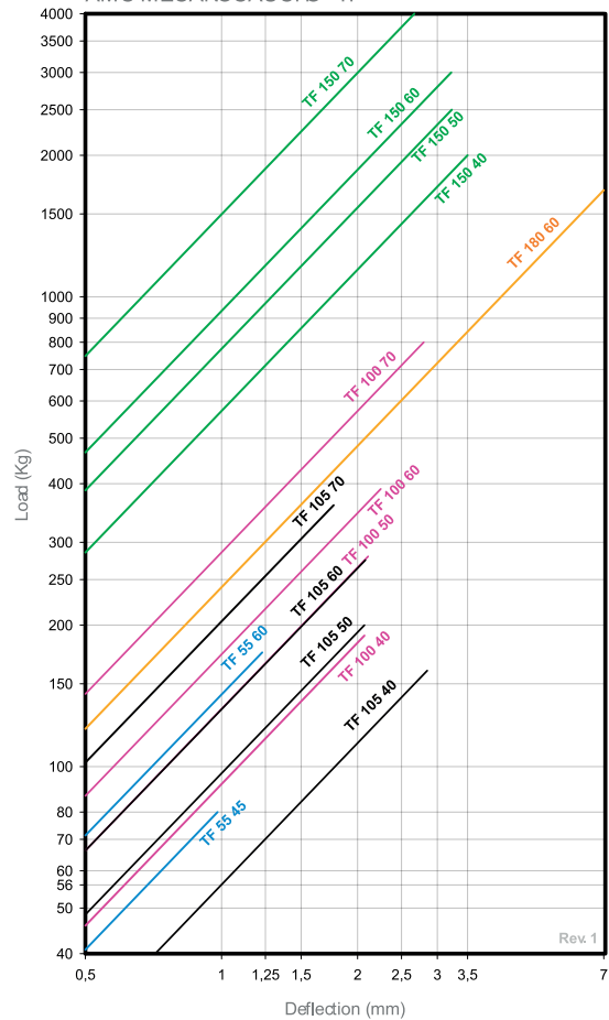
LOAD DEFLECTION GRAPHS AMC MECANOCAUCHO® TF
