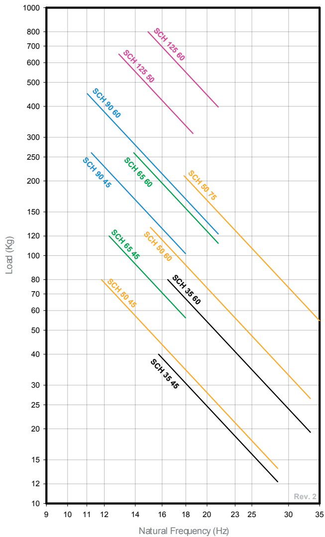
NATURAL FREQUENCY AMC MECANOCAUCHO® SCH
