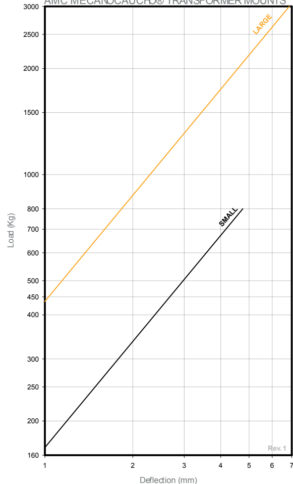
LOAD DEFLECTION GRAPH AMC MECANOCAUCHO® TRANSFORMER MOUNTS
