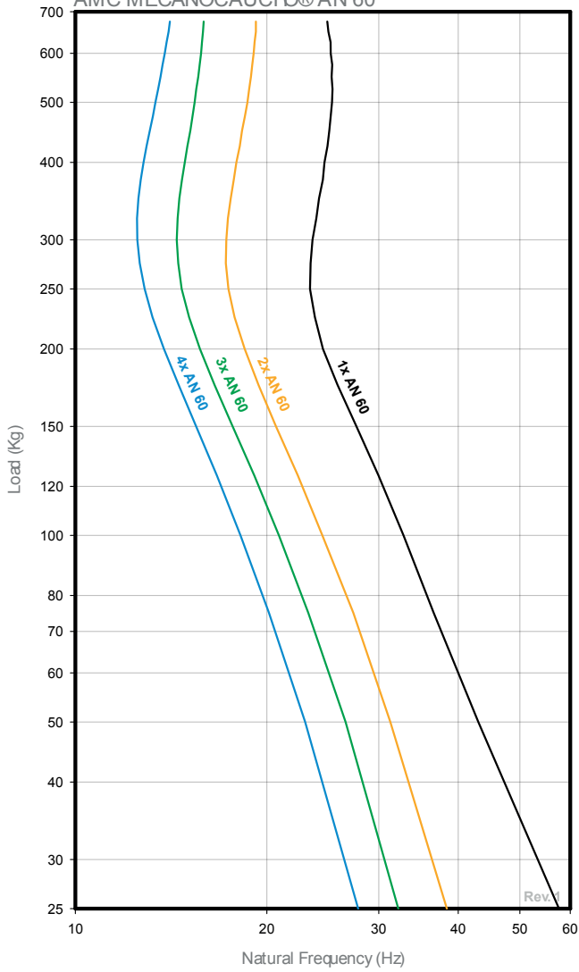
NATURAL FREQUENCY AMC MECANOCAUCHD® AN 60
