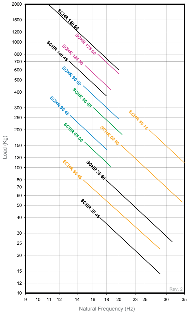
NATURAL FREQUENCY AMC MECANOCAUCHO® SCHR
