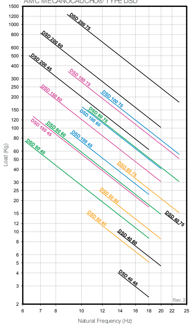
NATURAL FREQUENCY AMC MECANOCAUCHO® TYPE DSD
