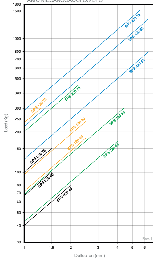
LOAD DEFLECTION GRAPH AMC MECANOCAUCHO® SPS
