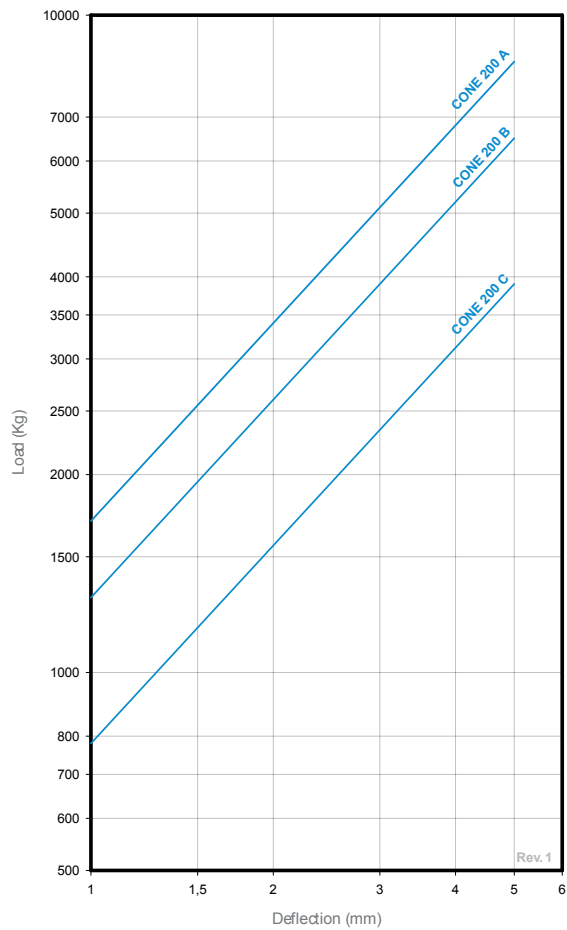
LOAD DEFLECTION GRAPH- AMC MECANOCACHO® CONE 200 WITH FIXATION FLANGE
