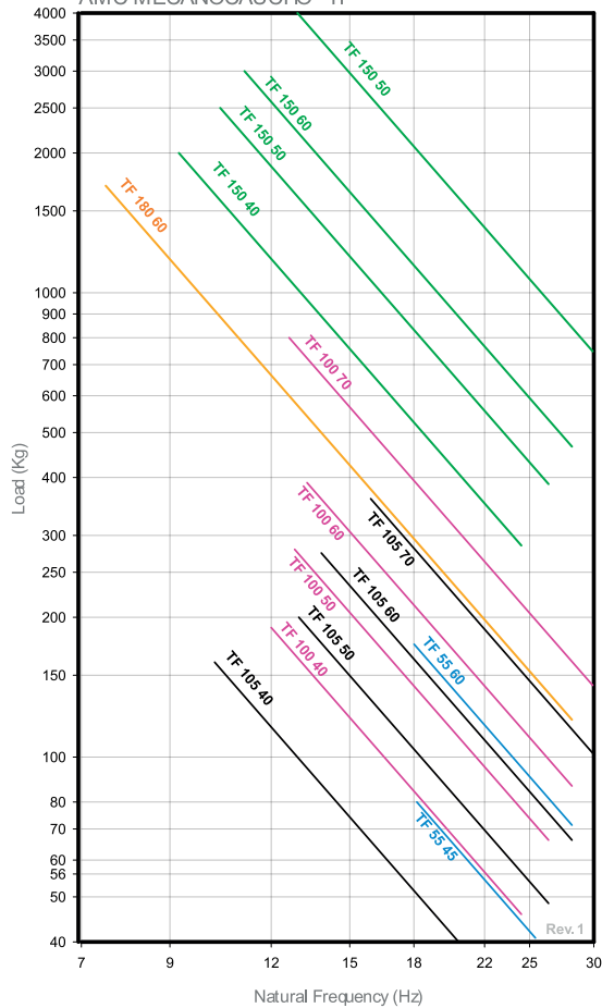
NATURAL FREQUENCY GRAPHS AMC MECANOCAUCHO® TF
