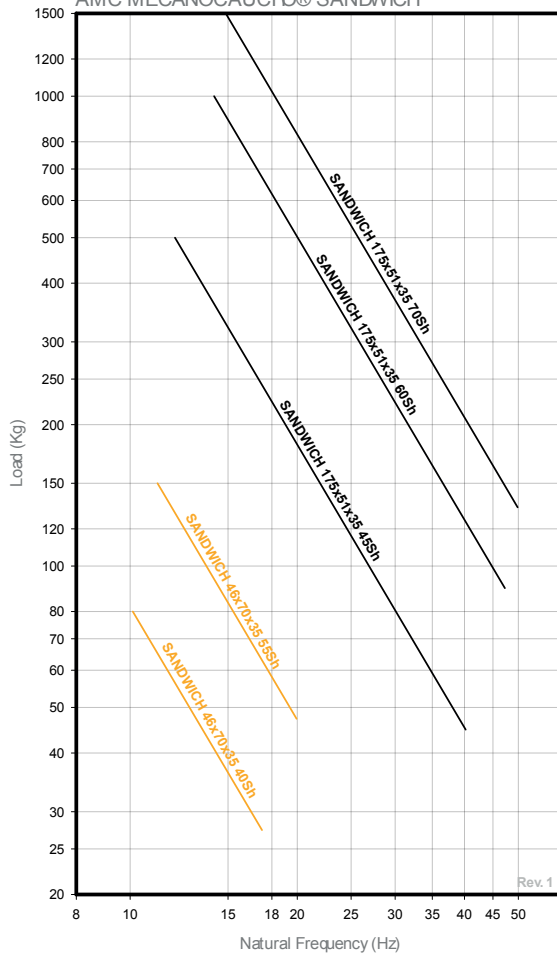
NATURAL FREQUENCY AMC MECANOCAUCHO® SANDWICH
