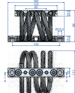
TYPE 160x89
