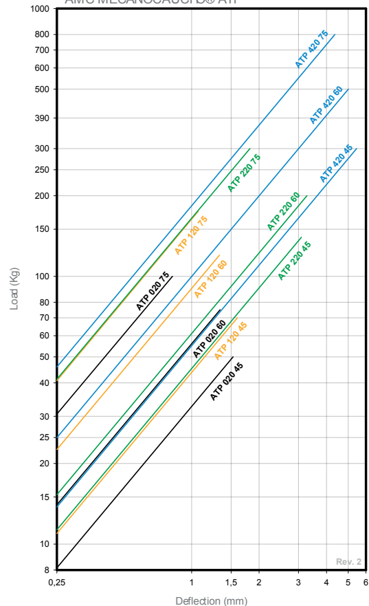
LOAD DEFLECTION GRAPH AMC MECANOCAUCHO® ATP
