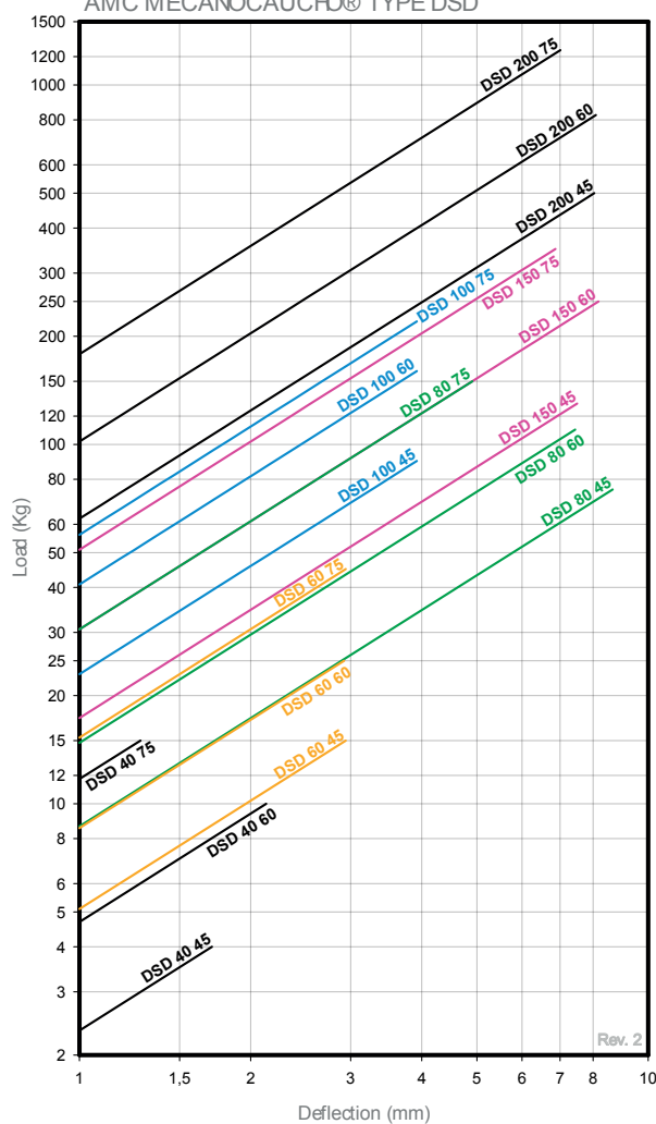
LOAD DEFLECTION GRAPH AMC MECANOCAUCHO® TYPE DSD
