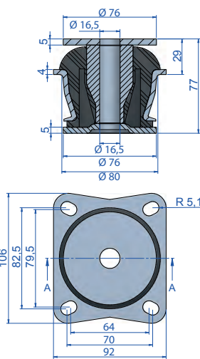
Top Washer Cone 30 code 608074 Lower Washer Cone 30 code 608125
