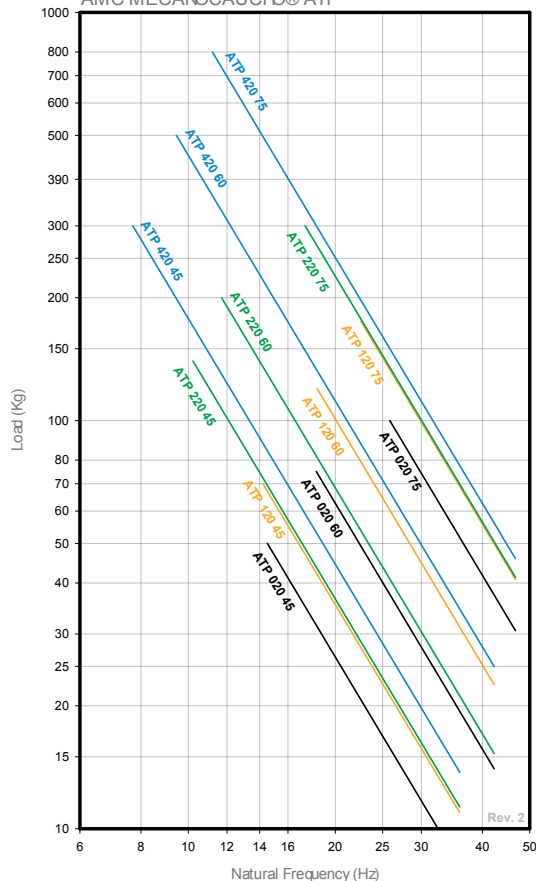
NATURAL FREQUENCY AMC MECANOCAUCHO® ATP
