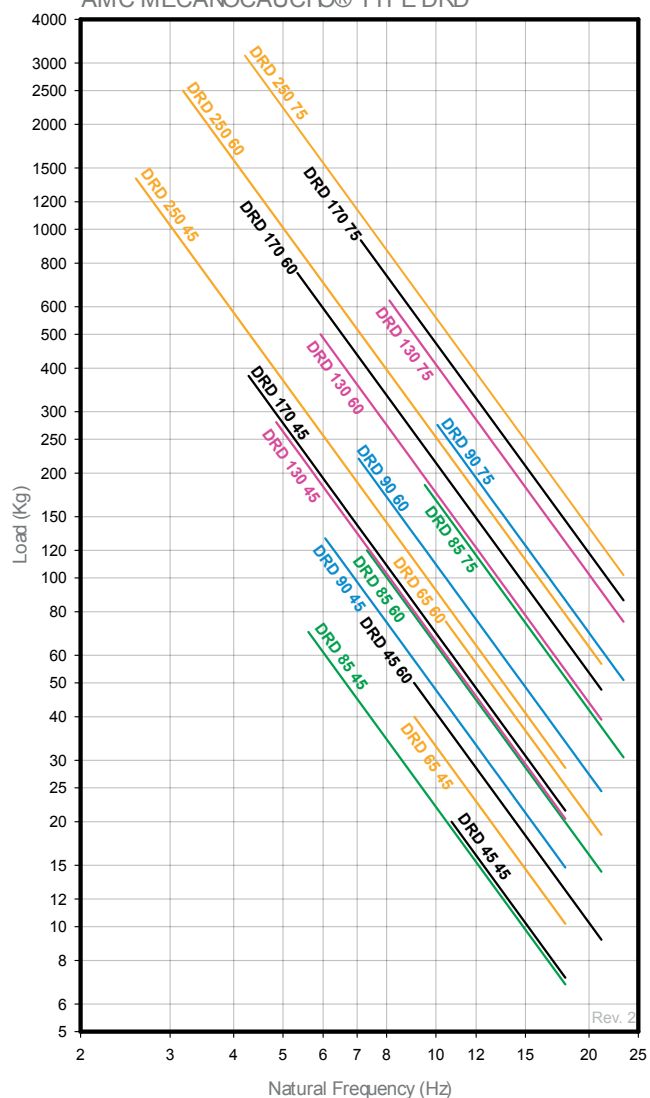
NATURAL FREQUENCY AMC MECANOCAUCHO® TYPE DRD
