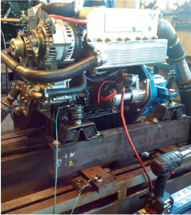
NATURAL FREQUENCY AMC MECANOCAUCHO® V-SHAPED MARINE MOUNT
