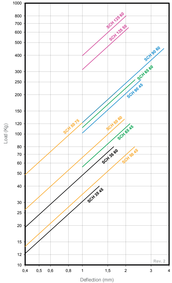
LOAD DEFLECTION GRAPH AMC MECANOCAUCHO® SCH
