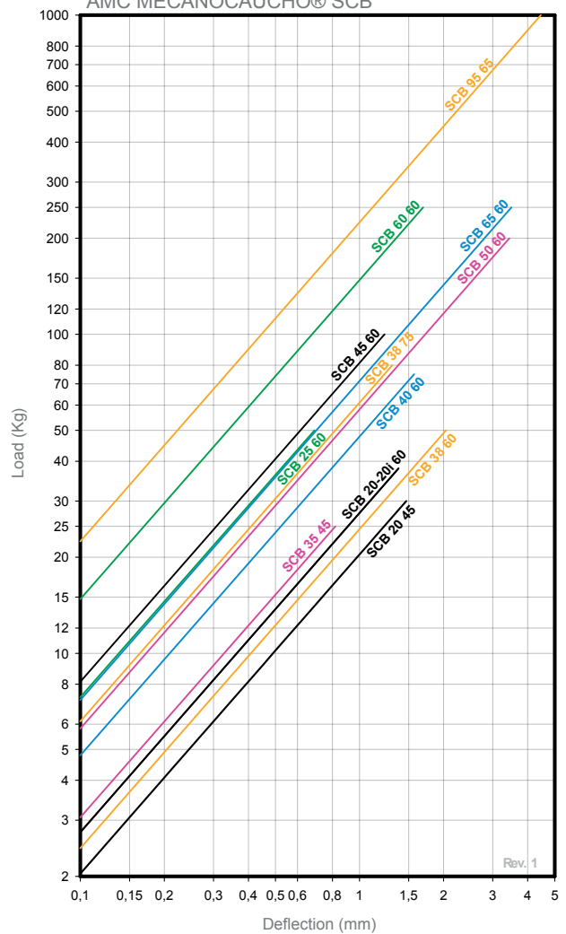
LOAD DEFLECTION GRAPH AMC MECANOCAUCHO® SCB
