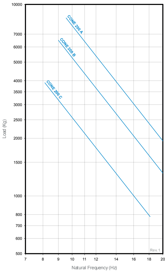
NATURAL FREQUENCY - AMC MECANOCACHO® CONE 200 WITH FIXATION FLANGE
