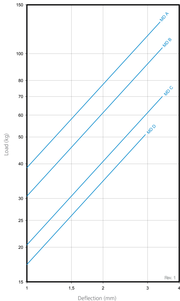
LOAD DEFLECTION GRAPH MECANOCAUCHO® MD TYPE
