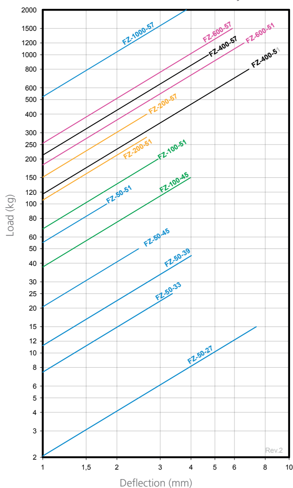
LOAD DEFLECTION GRAPH AMC MECANOCAUCHO® FZ + Sylomer®
